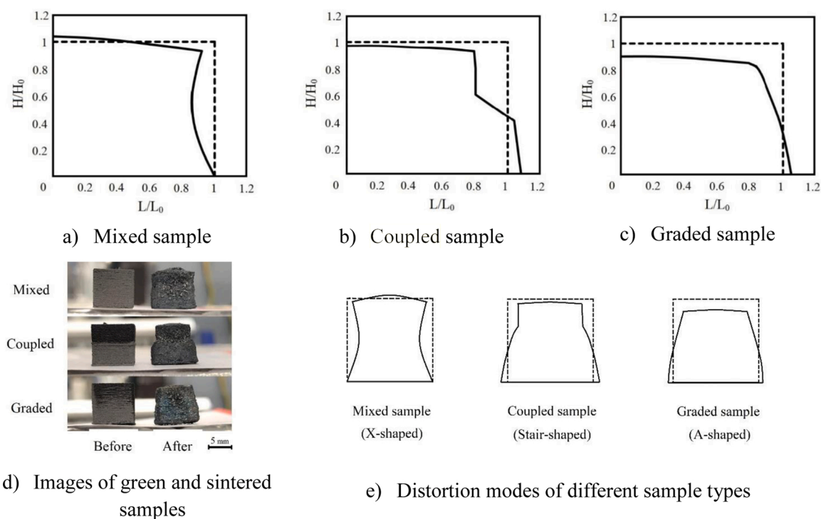
Fig. 8. The dimensional profiles of mixed (a), coupled (b), and graded (c) samples sintered at 1360 °C – 6 h – 0.2 °C/min. L/L 0 and H/H 0 are the sintered/green ratios (H 0 = 9.82 mm and L 0 = 5.28 mm). (d) the images and (e) the schematics of distortion modes before and after sintering.
