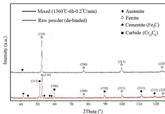
c) XRD patterns
