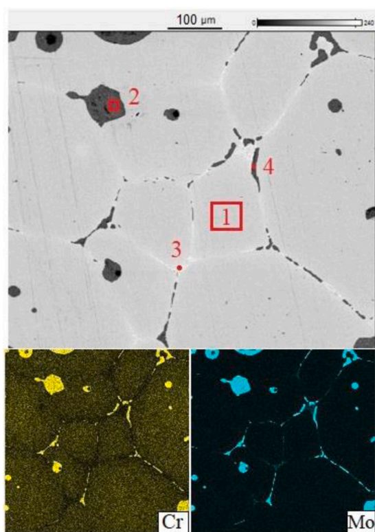
a) Mapping of Cr and Mo
